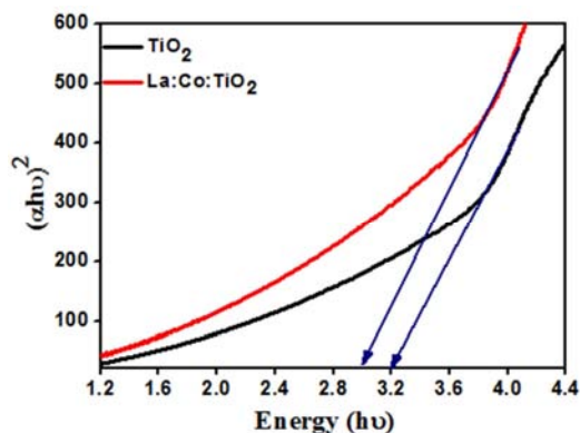
Figure 8. Band Gap energy of (a) \text{TiO}_2 (b) \text{La:Co:TiO}_2 .
