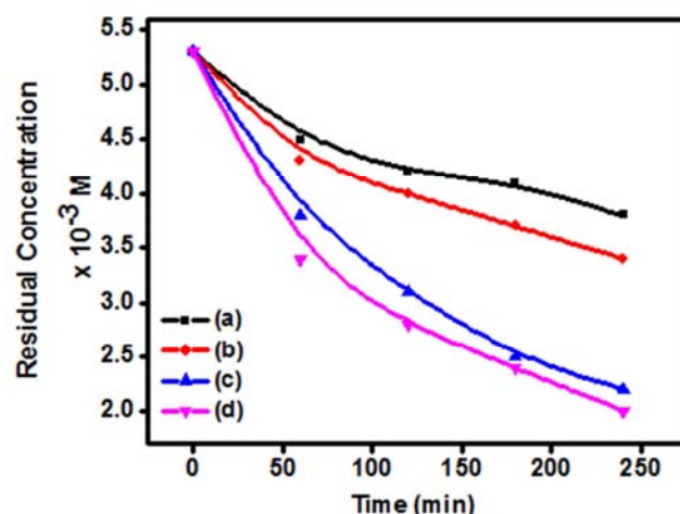
Figure 13. Photodegradation of Tartaric Acid at different amount (a) at 20g/l with TiO 2 (b) at 40g/l with TiO 2 (c) at 20g/l with La:Co:TiO 2 (d) at 40g/l with La:Co:TiO 2 .
