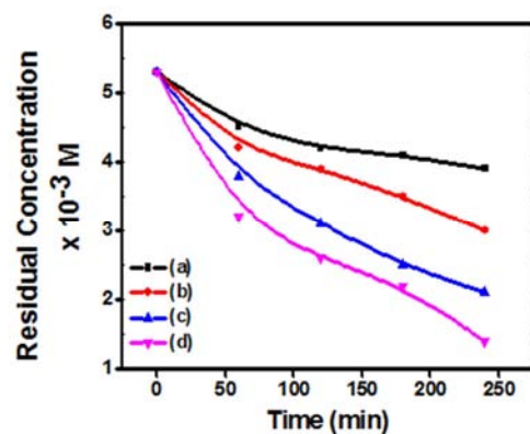
Figure 10. Effect of temperature on Photodegradation of Tartaric Acid (a) \text{TiO}_2 at 30°C (b) \text{TiO}_2 at 40°C (c) \text{La:Co:TiO}_2 at 30°C (d) \text{La:Co:TiO}_2 at 40°C.
