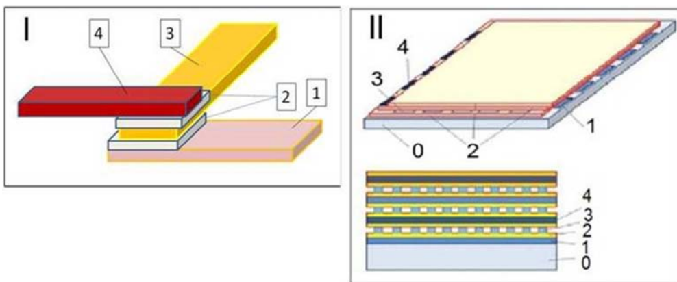
Figure 7. The scheme of storage cell (I) and storage spin media (II): 0 – substrate, 1 –first magnetic electrode, 2 –barrier nanolayer, 3 –second magnetic electrode, 4 –third magnetic electrode.
