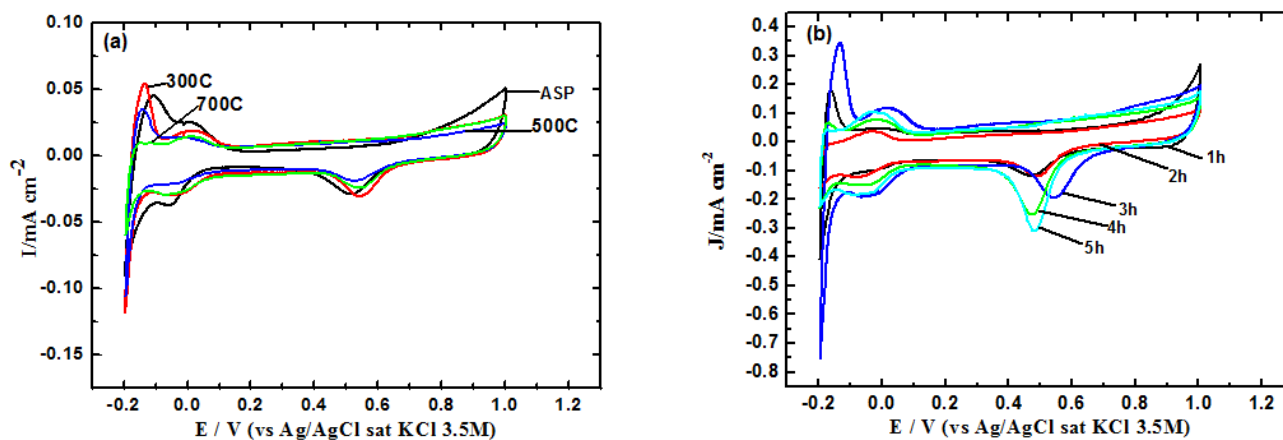
Fig. 3. Cyclic voltammograms of Pd-Fe/C catalysts (a) aged at different temperatures ASP (as prepared sample), 300 °C, 500 °C and 700 °C and (b) aged at 300 °C for different aging times 1h, 2h, 3h, 4h and 5h.
