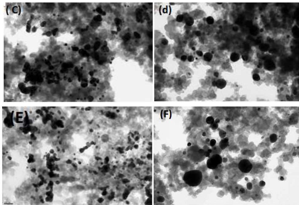
Fig. 2. TEM micrographs of the carbon-supported Pd-Fe (Pd:Fe = 70:30 atom%) (a) ASP sample and followed by aging for 3 h (b) at 300 °C; (c) at 500 °C and (d) at 700 °C, in (E) and (F) the studied sample aged at 300 °C for 1h and 5h respectively, all of these images with 100 nm magnification.
