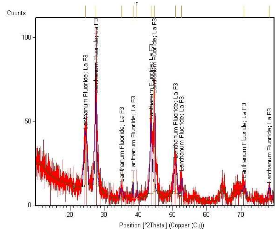
Figure 2. XRD spectra of \text{LaF}_3 deposited sample at room temperature.
